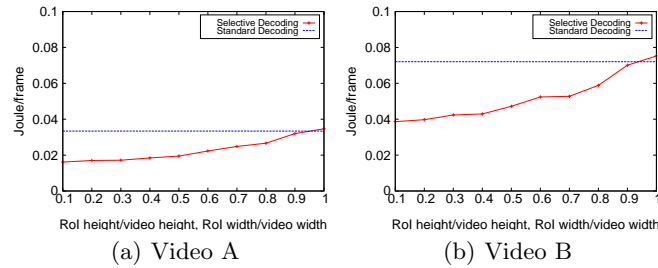
Fig. 9. CPU Power Consumption Per Frame
