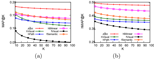
Figure 4: Performance of automatic image retrieval over the 95,800 queries.
