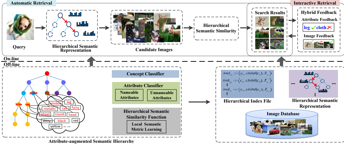
Figure 2: Illustration of the proposed Attribute-augmented Semantic Hierarchy (A 2 SH) and the image retrieval system developed on A 2 SH.
