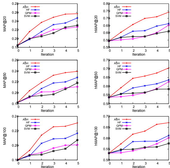
Figure 5: Performance of interactive retrieval with five feedback iterations over the 95,800 queries.
